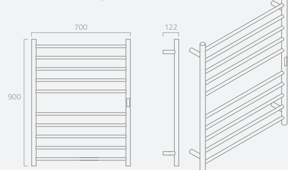
FLAT R10
