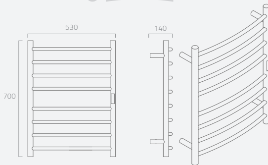
CURVE R8
