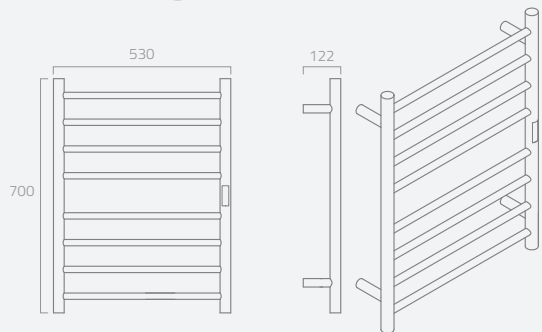
FLAT R8
